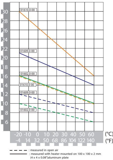
Heating Power in Relation to Ambient Temperature AC/DC 120 - 240 V
