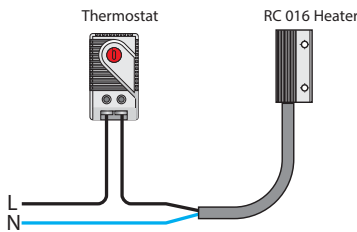
Wiring example
